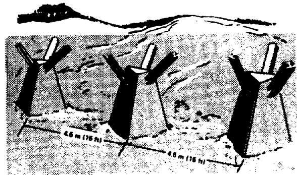
Figure 3-31. Horned scullies based on small dragon's teeth.
